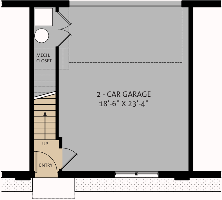
UNIT B ALLEY- LOWER LEVEL PLAN
